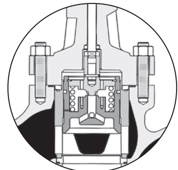
Model 41405 Pilot Balanced Construction FTC
