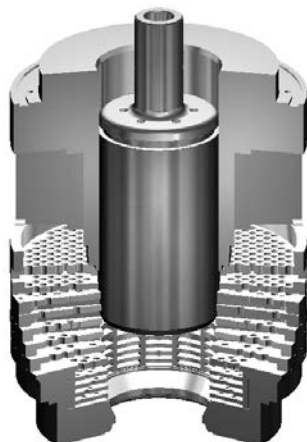
Model 41365 - 41375 High Pressure Anit-Cavitation VRT
